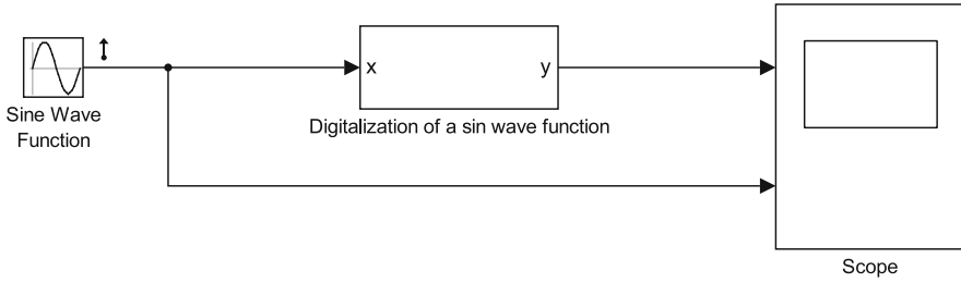
Fig. 5.8 Making the digitalization into a Simulink block
