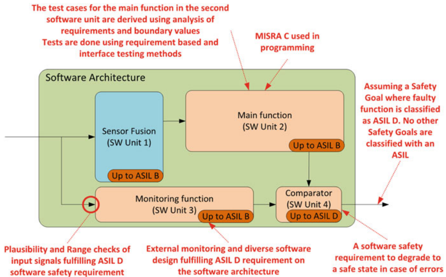
Fig. 8.10 A simple example of a software design for an assumed ASIL D Safety Goal
