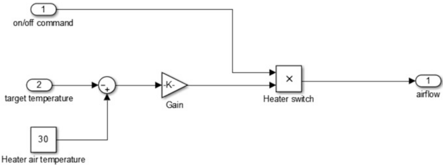
Fig. 5.19 Heater model
