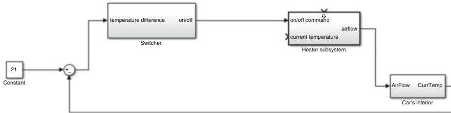
Fig. 5.24 First version of the air heater model with the feedback loop
